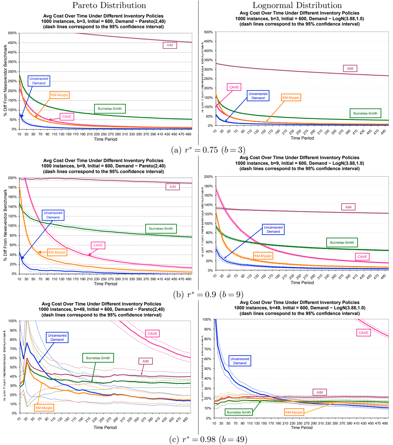
Figure 5 The running average cost under Pareto and Lognormal demand distributions.
