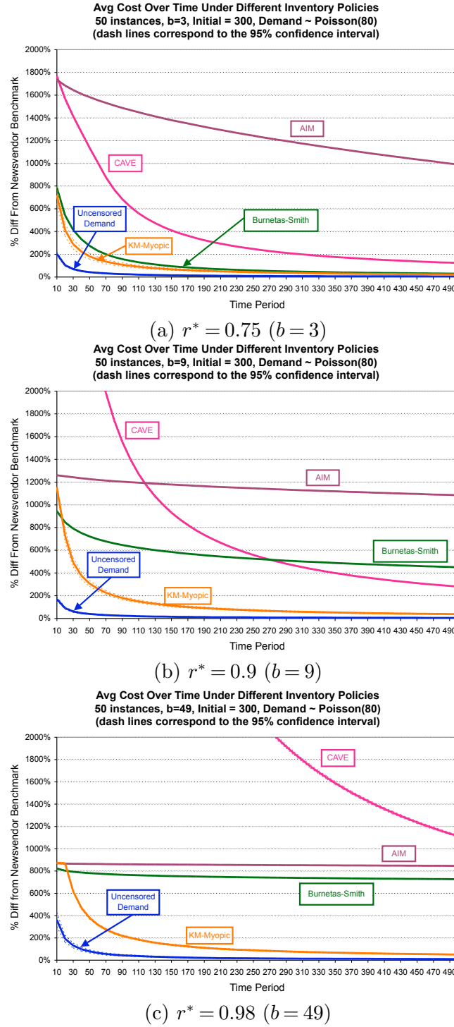
Figure 3 The percentage difference (compared to the newsvendor benchmark) of the running average cost over time under different inventory policies for 50 randomly generated problem instances for a Poisson demand distribution with mean 80 when the newsvendor quantile equals to 0.75, 0.9, and 0.98, respectively.
