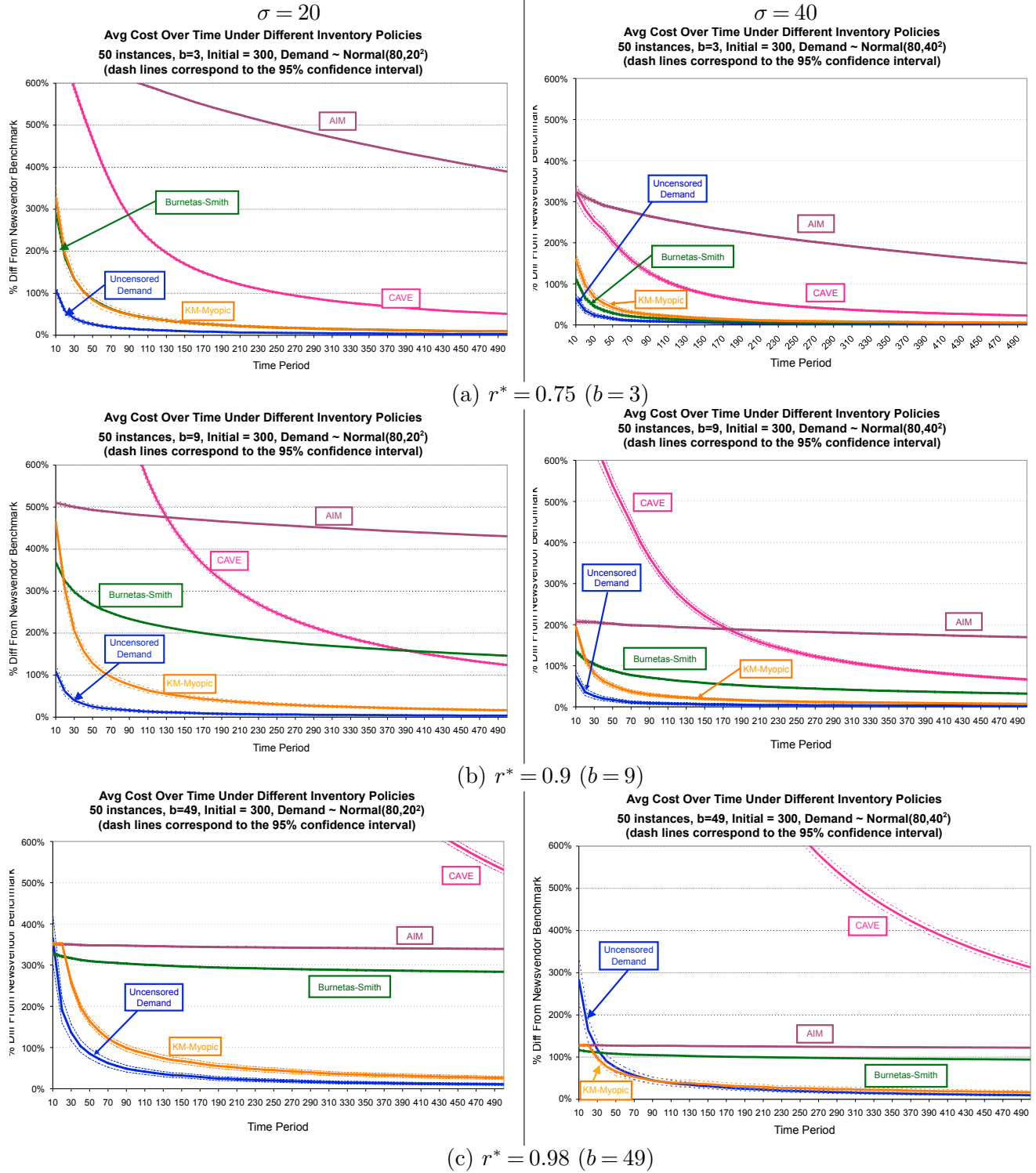
Figure 7 The running average cost under Gaussian demand distributions with increasing standard deviations.
