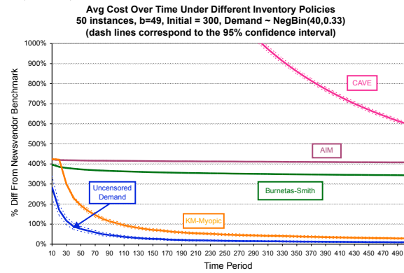
Figure 4 The running average cost under Negative Binomial demand distributions with increasing standard deviations.
