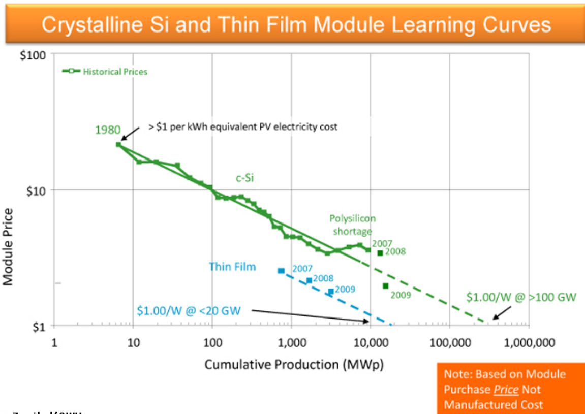
Figure 5. Solar Photovoltaic experience curve. Source: Ken Zweibel, George Washington University, http://solarcellcentral.com/cost_page.html ; see also http://solar.gwu.edu/Presentations/KZSolarContract.pdf .
