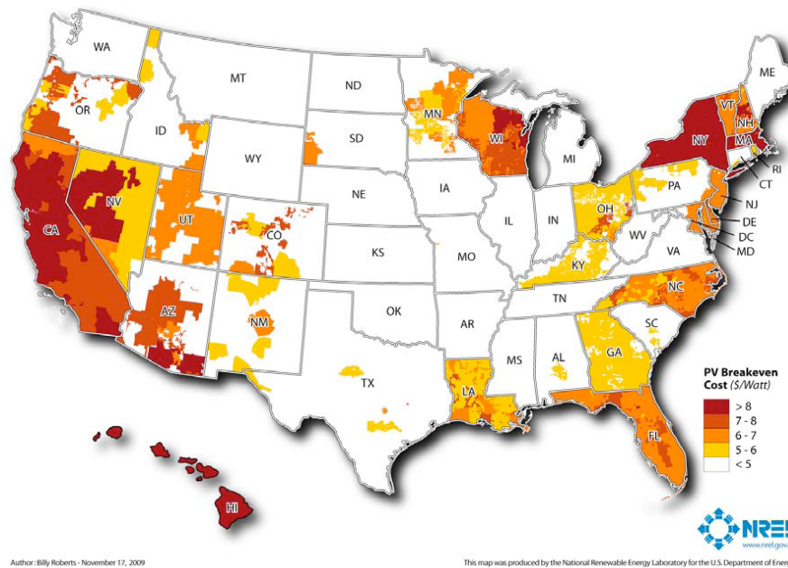
Figure 10. Heterogeneity in solar PV breakeven cost per peak watt in the United States due to variations in solar resource, local grid power prices and subsidies and tax credits for solar installation, as of 2008. Source: Denholm et al. (2009).
