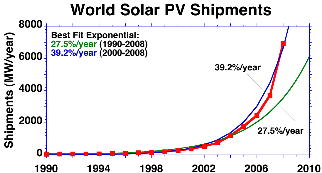
Figure 6. World Solar Photovoltaic Shipments, MW peak capacity/year. Source: PV News.
