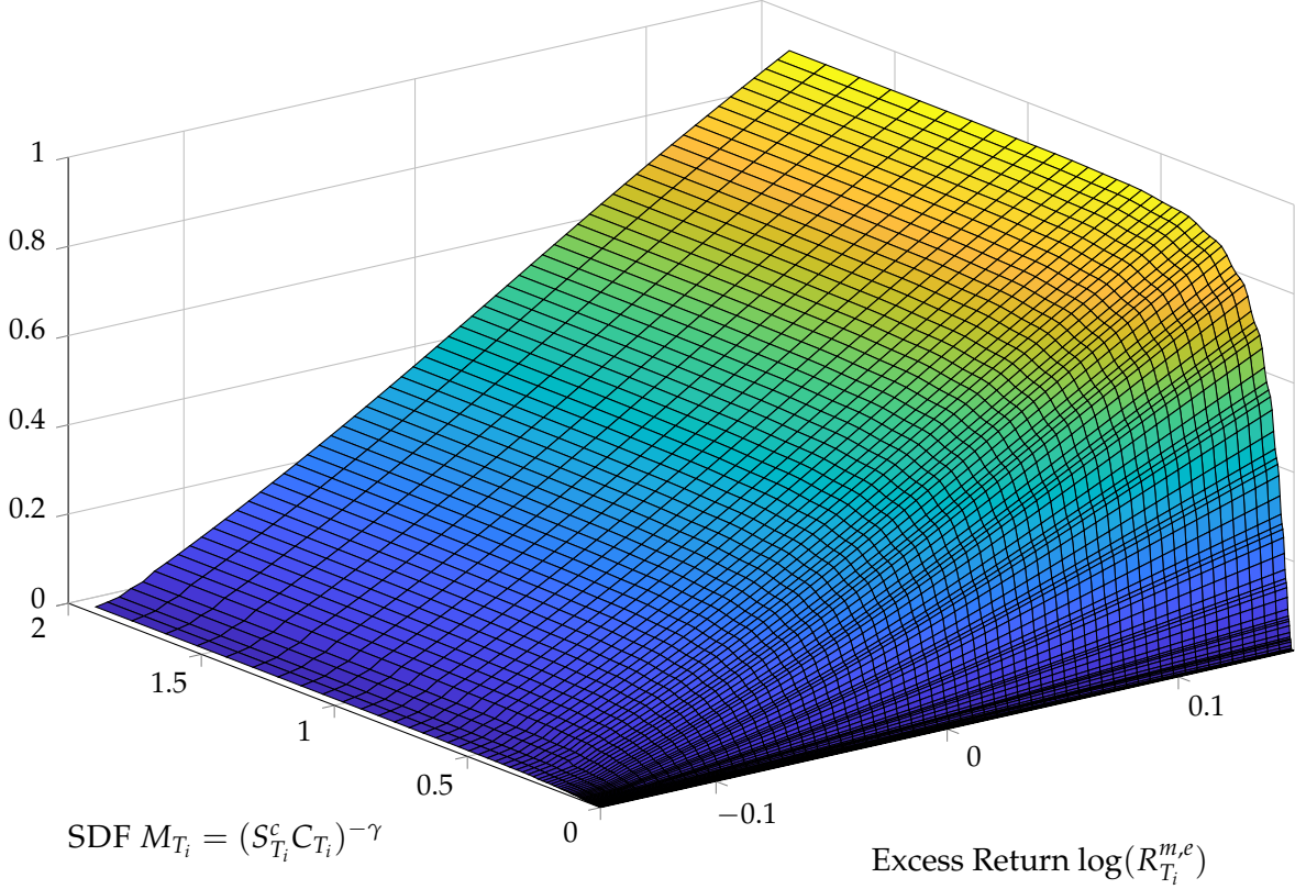
Figure B.1: Solution for Joint CDF for SDF and Return: Example at S_t^c = \bar{S}^c , t = 0_i
