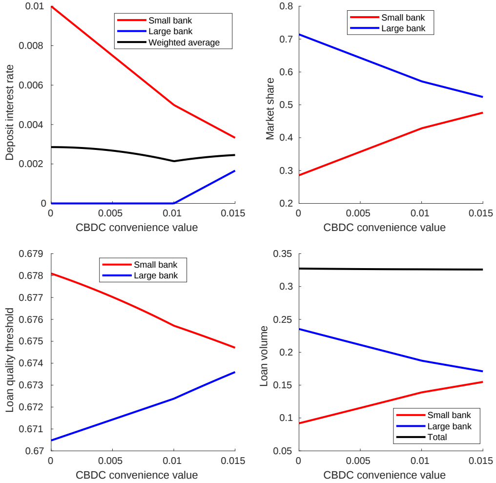
Figure 2: Impact of CBDC convenience value on deposit and lending markets. Parameters: G(\delta) = \delta/0.035 , A = 1.5 , X = 10 , f = 0.02 , s = 0 .
