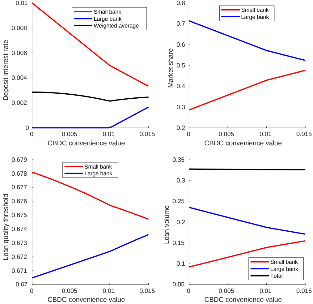
Figure 2: Impact of CBDC convenience value on deposit and lending markets. Parameters: G(\delta) = \delta/0.035 , A = 1.5 , X = 10 , f = 0.02 , s = 0 . The equilibrium transitions from constrained to unconstrained at v = 0.01 .
