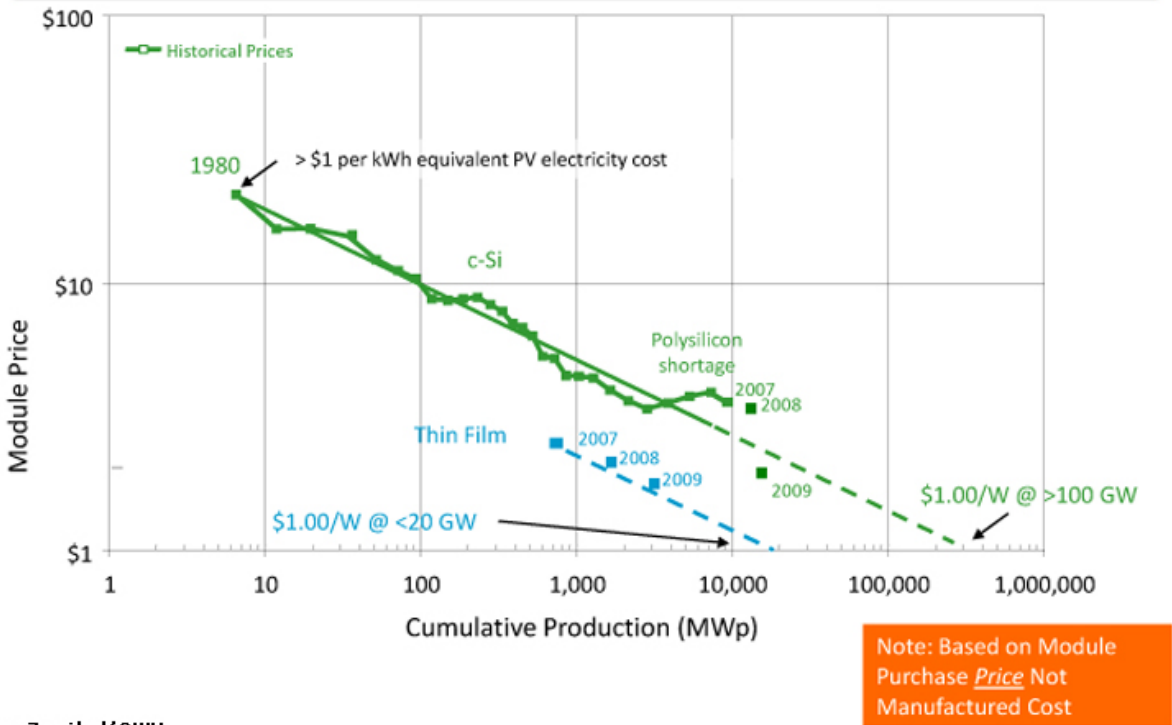
Figure 5. Solar Photovoltaic experience curve. Source: Ken Zweibel, George Washington University, http://solarcellcentral.com/cost_page.html ; see also http://solar.gwu.edu/Presentations/KZSolarContract.pdf .
