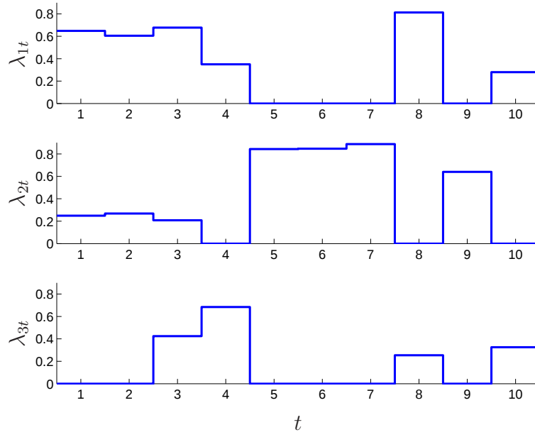
Figure 7: Optimal link prices.
