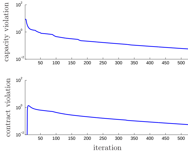
Figure 3: Maximum link capacity violation (top) and contract violation (bottom), versus iteration.
