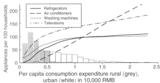
FIGURE 2. ADOPTION OF APPLIANCES BY TYPE VERSUS CONSUMPTION EXPENDITURE
