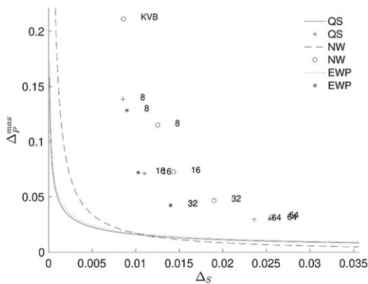
FIGURE S2.—Theoretical (lines) and Monte Carlo (symbols) size distortion/power loss for QS, Newey–West, and EWP tests. Stochastic regressor, m = 1 , AR(1), \rho = 0.5 , T = 200 . Theoretical curves are for the Gaussian location model.
