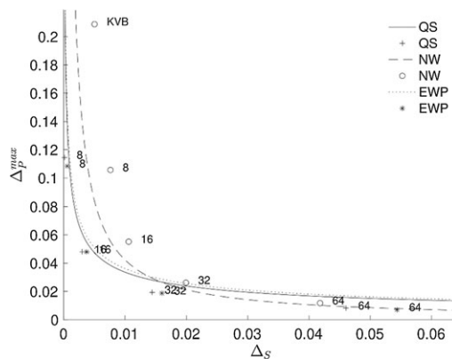
FIGURE S1.—Theoretical (lines) and Monte Carlo (symbols) size distortion/power loss for QS, Newey–West, and EWP tests. Location model, m=1 , AR(1), \rho=0.5 , and T=200 .
